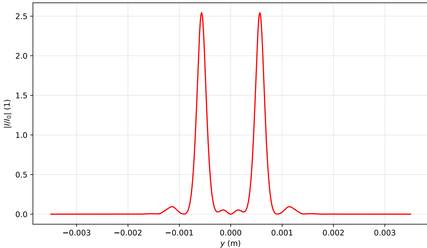
Intensity profile I(x=0, y, z=0.876)/I_0 , \text{Pin}=9.0\text{Pcr} , artificial time
